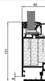
door with low-level threshold, bottom view
